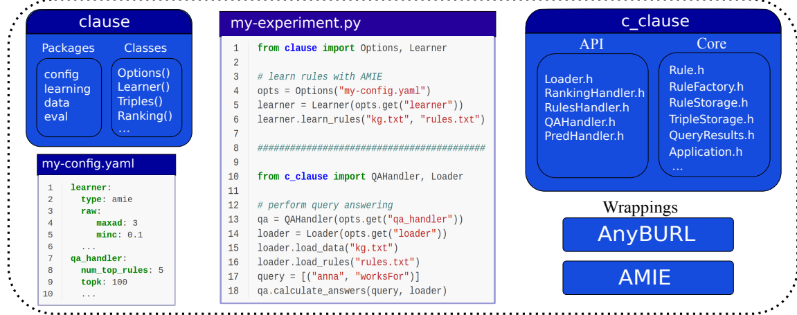
Figure 1: Usage-centric library overview.
