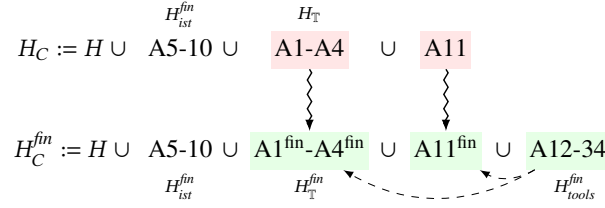
Fig. 2. Overview of the process of finite axiomatization. Zigzag arrows indicate the finite sets are counterparts to the top infinite ones. Dotted arrows indicate the the elements of H_{tools}^{fin} are used to define said counterparts.
